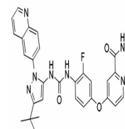
Chemical structure of DCC-2036 (Rebastin...)
