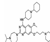
Chemical structure of UNC0646
