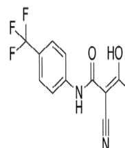
Chemical structure of Teriflunomide(A-77...
