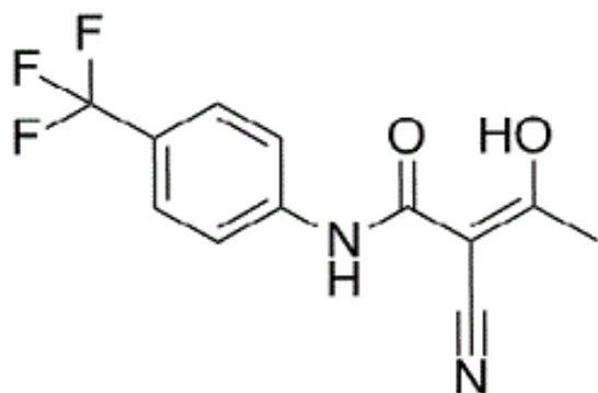
Chemical structure of Teriflunomide(A-771726).
