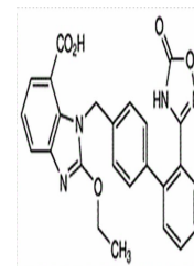
Chemical structure of Azilsartan kamedoxomil
