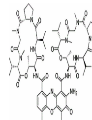
Chemical structure of Actinomycin D
