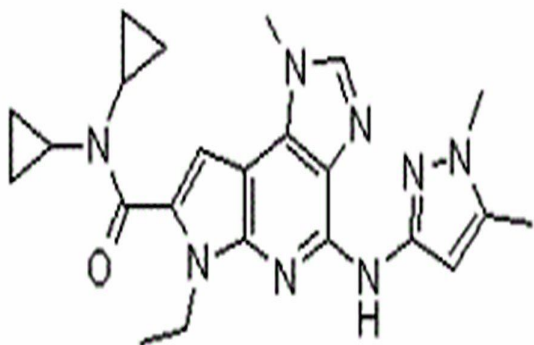
Chemical structure of BMS-911543
