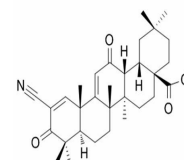
Chemical structure of Bardoxolone methyl
