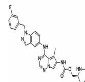
Chemical structure of BMS-599626 (AC480)
