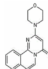
Chemical structure of Compound 401
