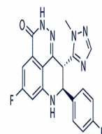
Chemical structure of Talazoparib(BMN-673)
