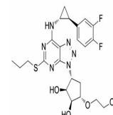
Chemical structure of Ticagrelor (Brilinta)
