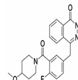
Chemical structure of AZD2461
