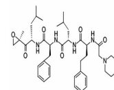
Chemical structure of Carfilzomib
