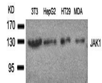
Western blot analysis of JAK1(Ab-1022) a...
