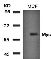
Western blot analysis of Myc(Ab-58) anti...
