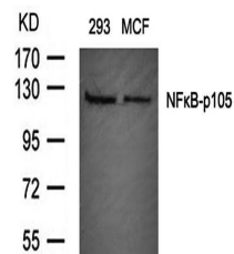
Western blot analysis of NFκB-p105(Ab-907) in 293 and MCF cell lines.
