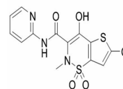
Chemical structure of Lornoxicam
