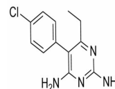
Chemical structure of Pyrimethamine
