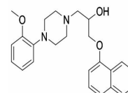
Chemical structure of Naftopidil
