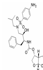
Chemical structure of Darunavir
