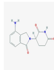
Chemical structure of Lenalidomide
