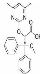
Chemical structure of Ambrisentan
