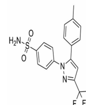
Chemical structure of Celecoxib
