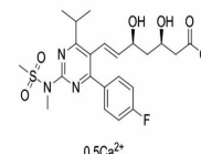
Chemical structure of Rosuvastatin Calcium
