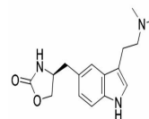
Chemical structure of Zolmitriptan
