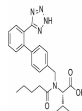
Chemical structure of Valsartan
