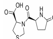
Chemical structure of Pidotimod
