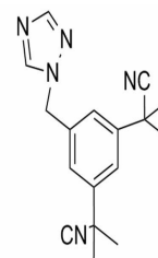
Chemical structure of Anastrozole
