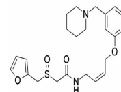
Chemical structure of Lafutidine
