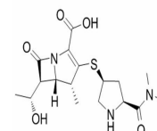
Chemical structure of Meropenem
