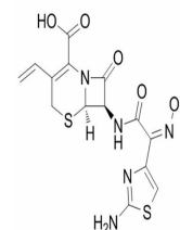
Chemical structure of Cefdinir (Omnicef)
