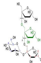
Chemical structure of Inulin
