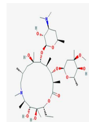
Chemical structure of Azithromycin
