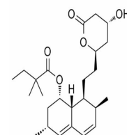
Chemical structure of Simvastatin (Zocor...)
