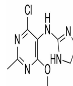
Chemical structure of Moxonidine
