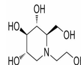
Chemical structure of Miglitol (Glyset)
