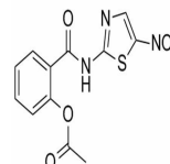
Chemical structure of Nitazoxanide (Alin...
