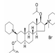
Chemical structure of Vecuronium Bromide
