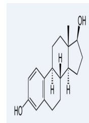
Estradiol chemical structure
