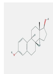
Chemical structure of Estradiol; beta- Es...
