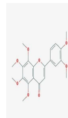
Chemical structure of nobiletin
