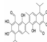
Chemical structure of Gossypol
