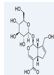
Geniposidic acid chemical structure
