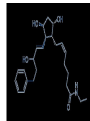
Chemical structure of Bimatoprost
