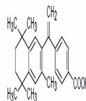
Chemical structure of Bexarotene
