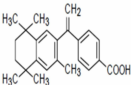
Chemical structure of Bexarotene
