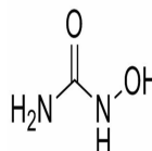
Chemical structure of Hydroxyurea (Cytod...
