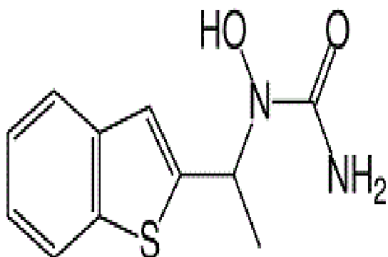
Chemical structure of Zileuton.
