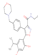
Structure of Luminespib.
