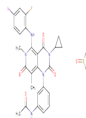
Chemical structure of Trametinib (DMSO s...
