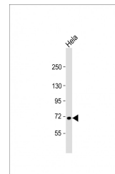
Western Blot at 1:2000 dilution + Hela w...
