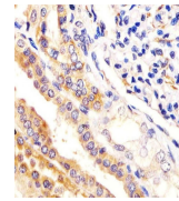
Antibody staining USP2 in human kidney t...
