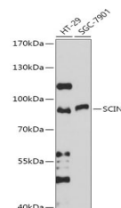
Western blot analysis of extracts of var...
